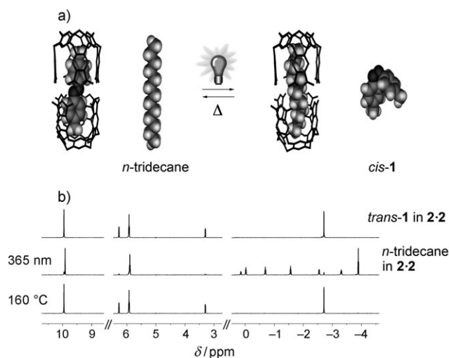
Figure 1. a) Light-induced guest exchange of trans - 1 by n -tridecane in 2 · 2 . b) Indicative regions of the 1 H NMR spectra ([D 12 ]mesitylene, 20 °C) are shown before irradiation ( trans - 1 is the only guest) and after irradiation at 365 nm wavelength for 50 min at 20 °C ( n -tridecane is the only guest). After heating the sample to 160 °C for 2 min, the initial state was completely restored.
